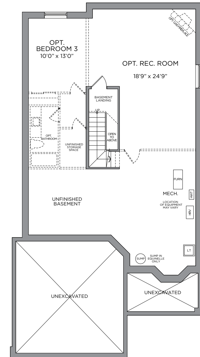
STANDARD BASEMENT PLAN OPT. FINISHED BASEMENT 812 SQ. FT.
