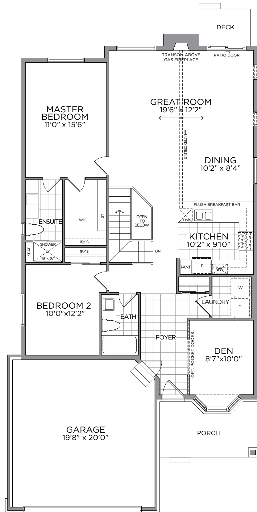
GROUND FLOOR ELEV. B
