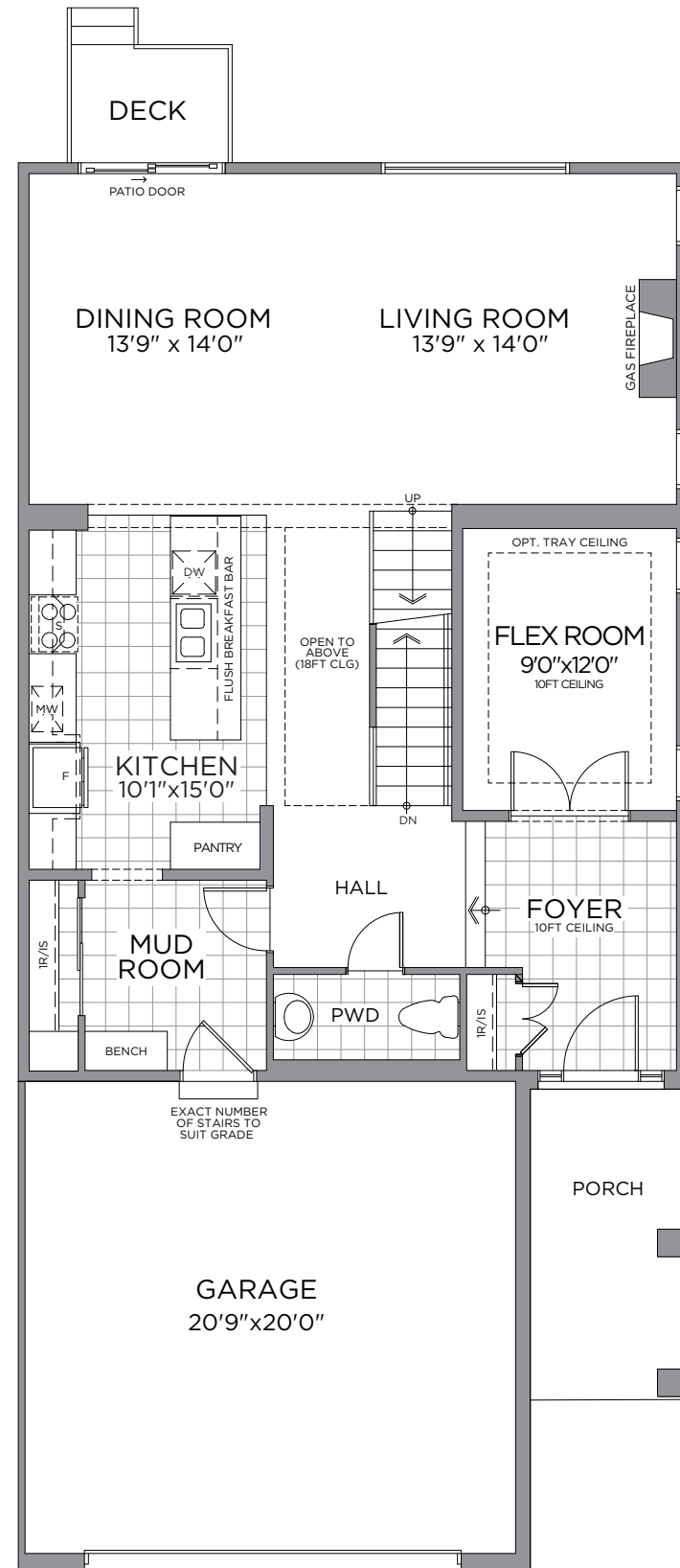
GROUND FLOOR
