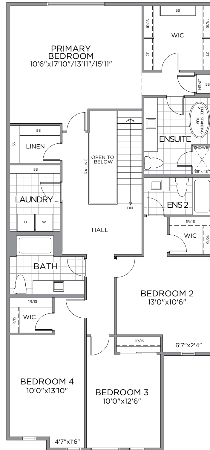
SECOND FLOOR
