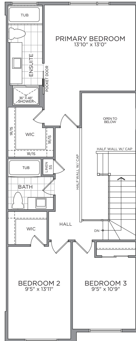
SECOND FLOOR
