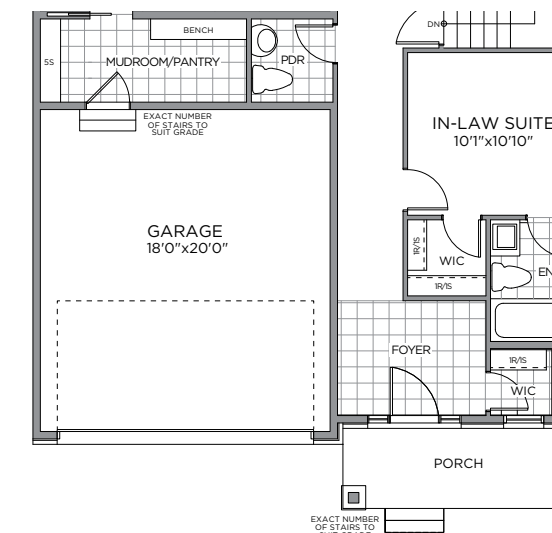
OPT. GROUND FLOOR PLAN W/ IN-LAW SUITE ELEV. B
