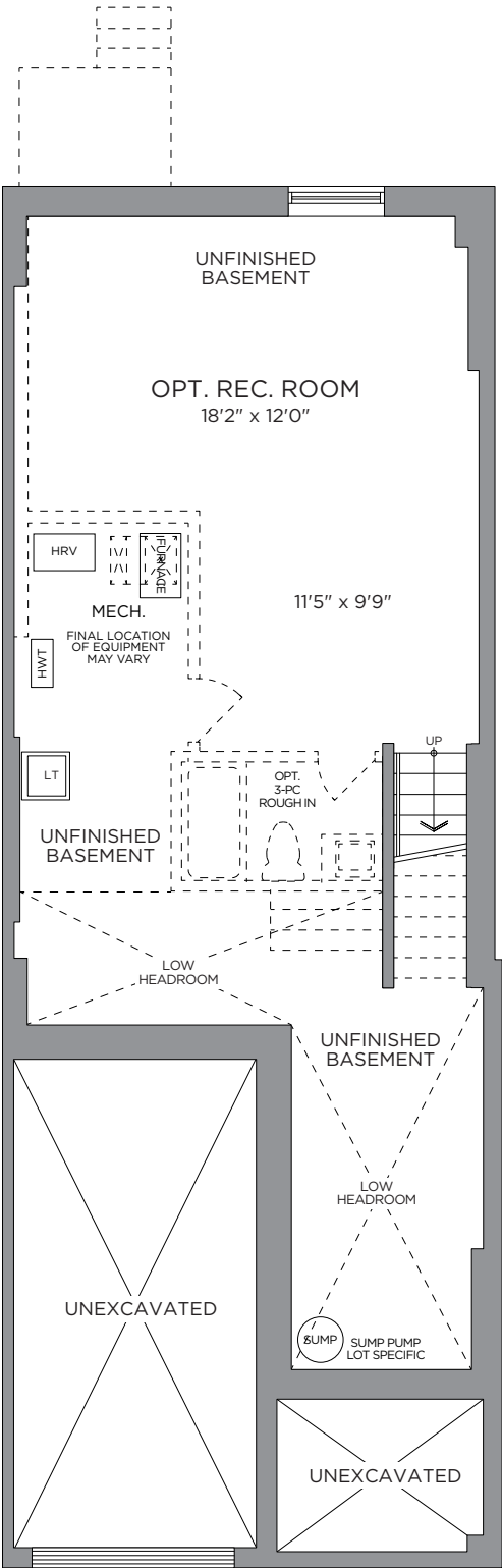
STANDARD BASEMENT OPT. FINISHED BASEMENT REC. ROOM 392 SQ. FT.
