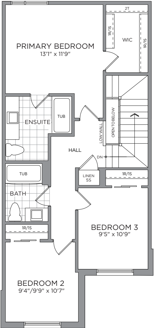
SECOND FLOOR
