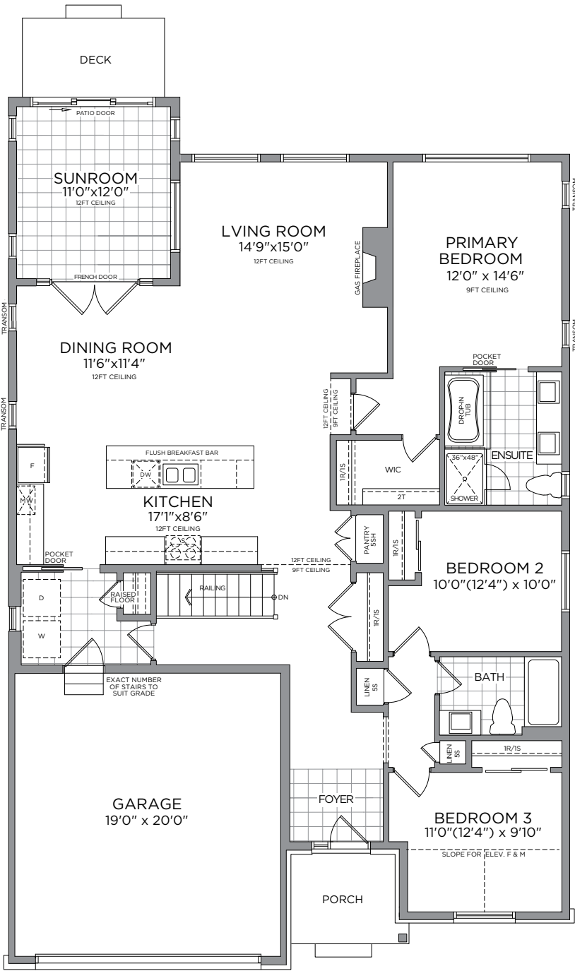
GROUND FLOOR
