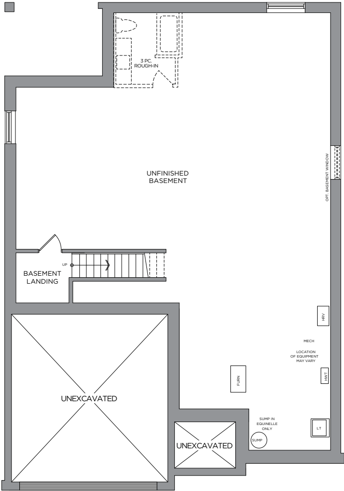
BASEMENT
