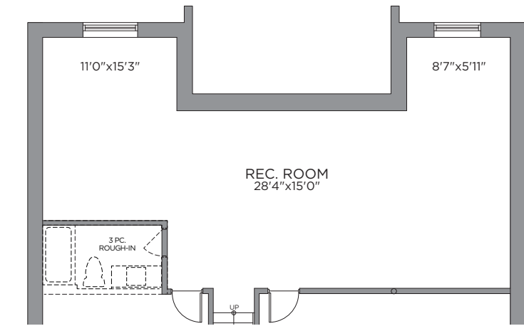
OPT. FINISHED BASEMENT REC. RM. 771 SQ. FT.
