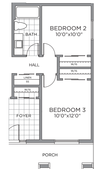
OPT. 3 BEDROOM PLAN GROUND FLOOR
