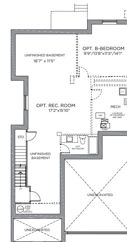
STANDARD BASEMENT PLAN OPT. FINISHED BASEMENT PLAN 1074 SQ. FT.
