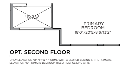
ONLY ELEVATION "B", "M" & "F" COME WITH A SLOPED CEILING IN THE PRIMARY. ELEVATION "C" PRIMARY BEDROOM HAS A FLAT CEILING AT 8'.
