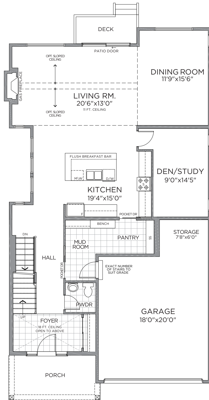
GROUND FLOOR
