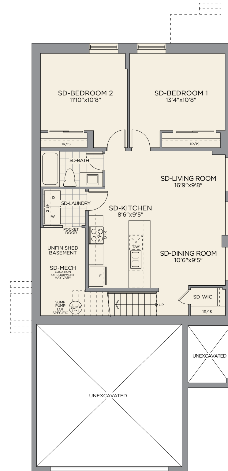
STANDARD BASEMENT PLAN (SECONDARY SUITE)
