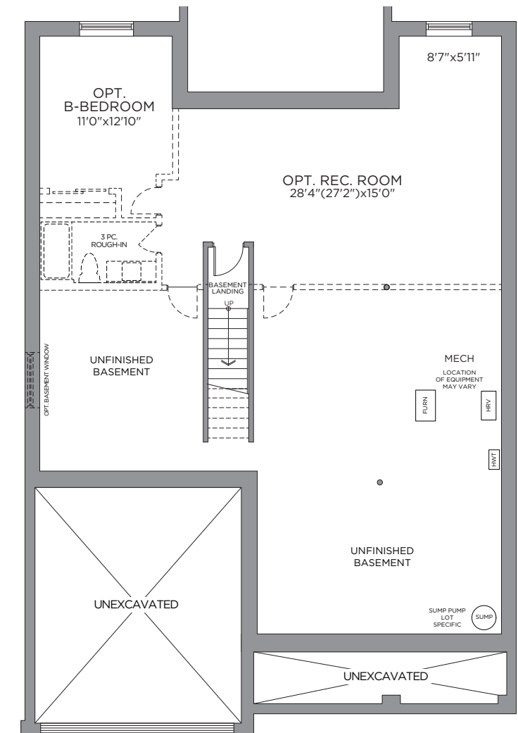
STANDARD BASEMENT PLAN OPT. FINISHED BASEMENT 836 SQ. FT.
