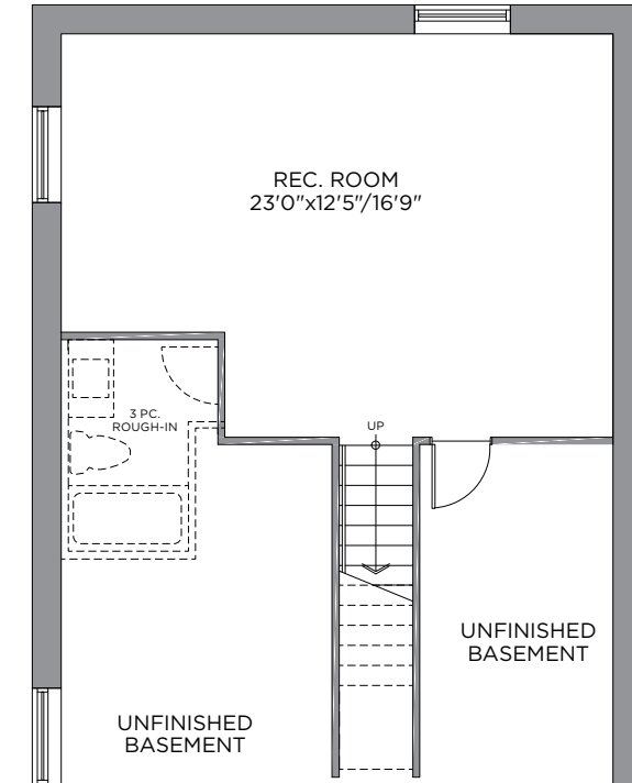
OPT. FINISHED BASEMENT REC. RM. 427 SQ. FT.
