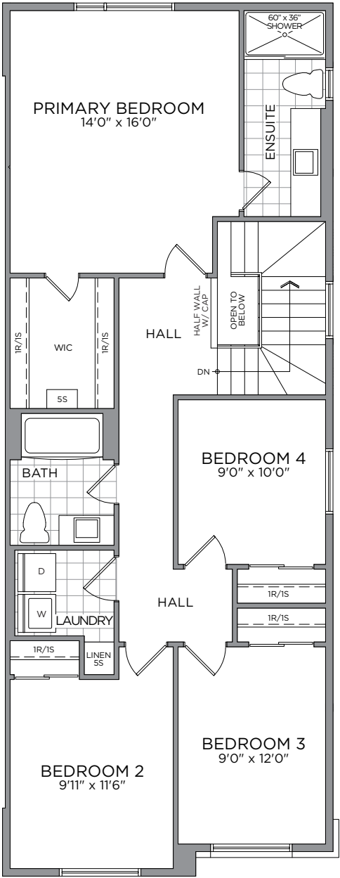
SECOND FLOOR
