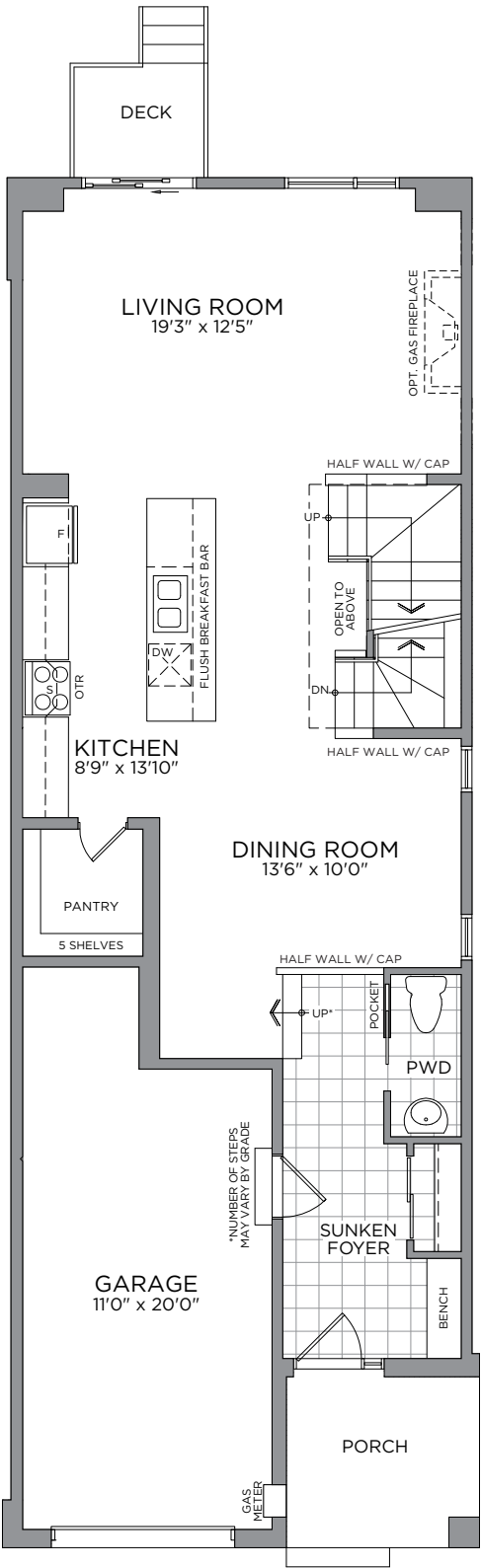
GROUND FLOOR
