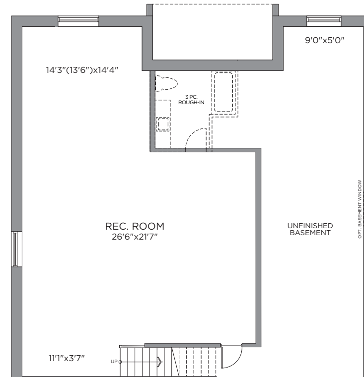
OPT. FINISHED BASEMENT REC. ROOM 922 SQ. FT.
