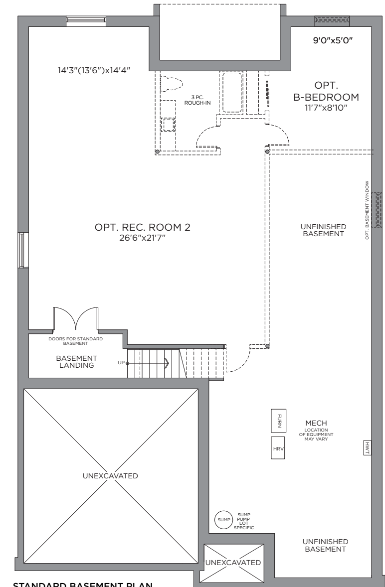
STANDARD BASEMENT PLAN OPT. FINISHED BASEMENT PLAN 1,245 SQ. FT.
