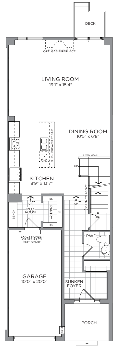
GROUND FLOOR
