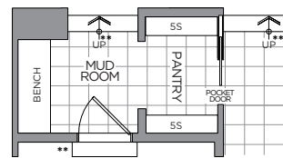
GROUND FLOOR WITH PANTRY PASS THROUGH
