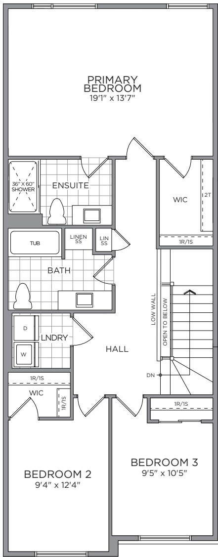
SECOND FLOOR
