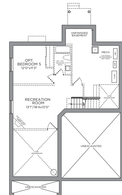
STANDARD BASEMENT OPT. FINISHED BASEMENT FINISHED AREA 503 SQ. FT.
