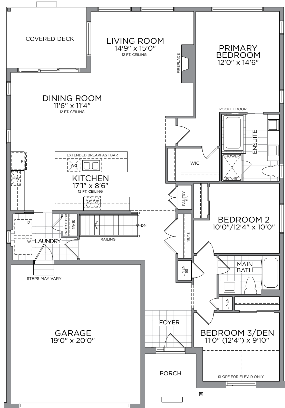
GROUND FLOOR
