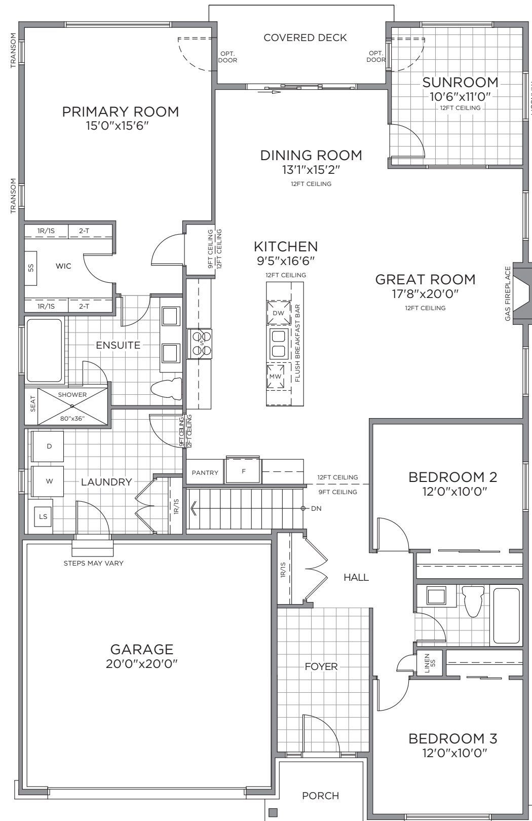
GROUND FLOOR ELEV. B/D
