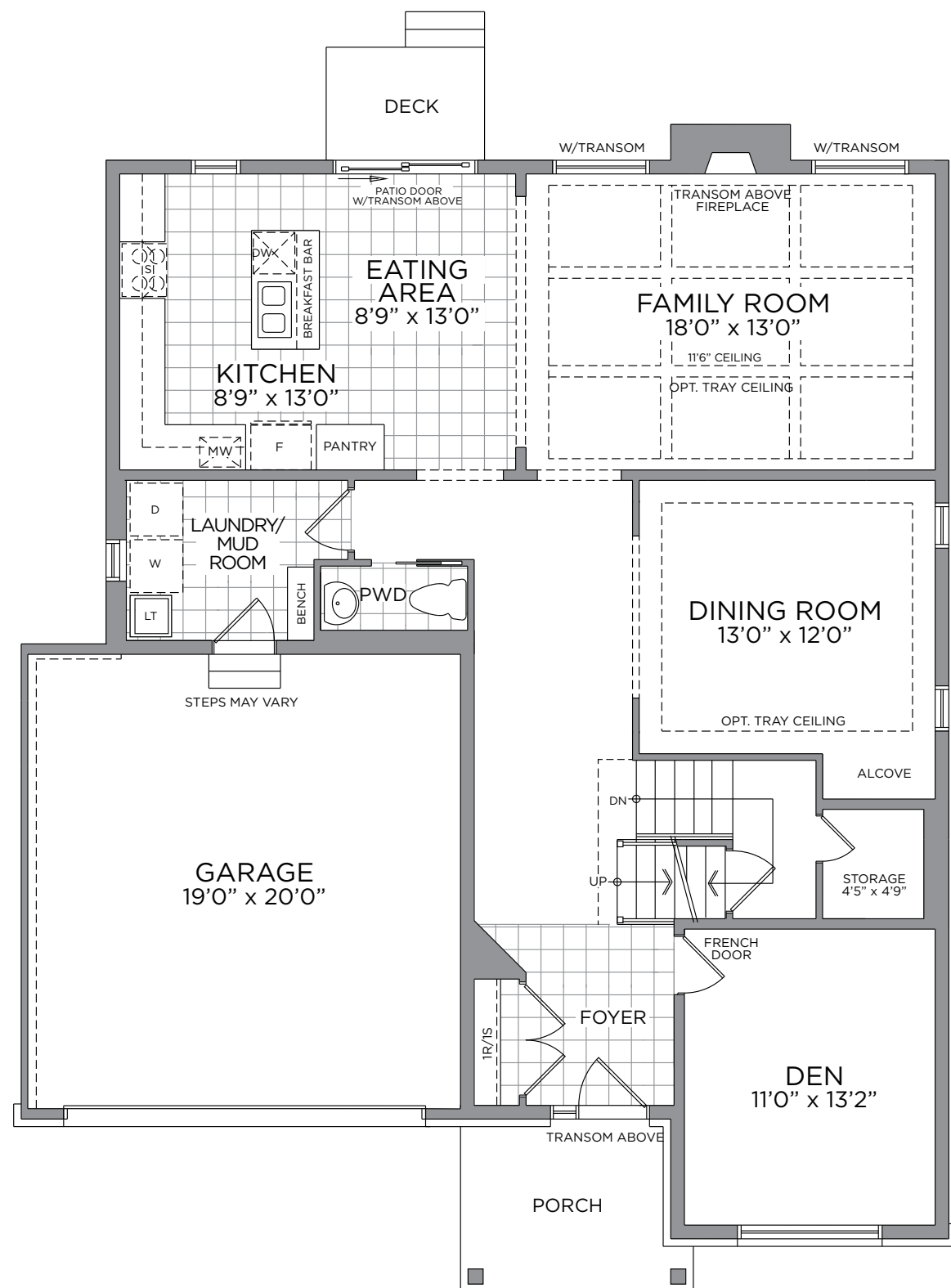
GROUND FLOOR ELEV. B
