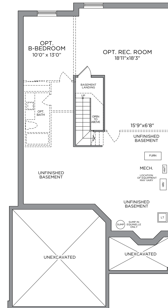
STANDARD BASEMENT OPT. FINISHED BASEMENT 808 SQ. FT.
