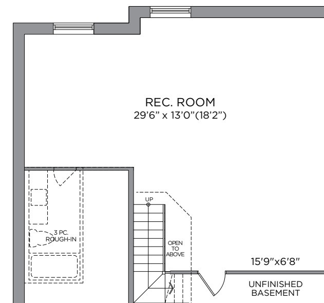
OPT. FINISHED BASEMENT REC. ROOM 687 SQ. FT.
