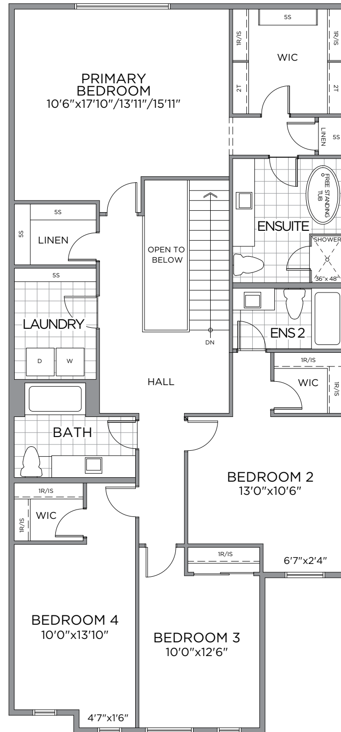
SECOND FLOOR
