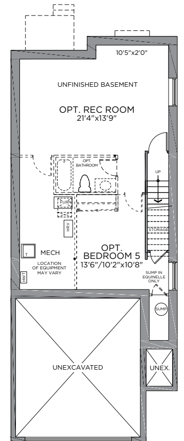
STANDARD BASEMENT PLAN ELEVATION C
