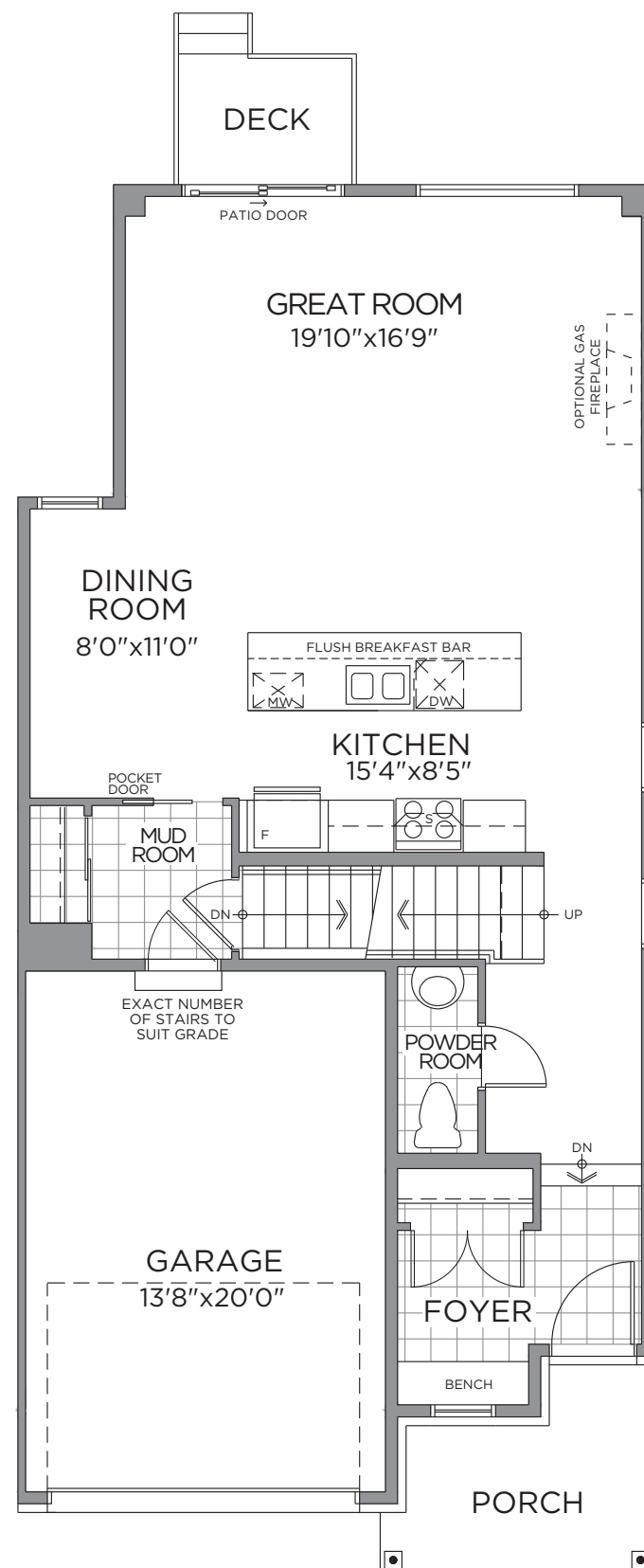
GROUND FLOOR ELEV. B
