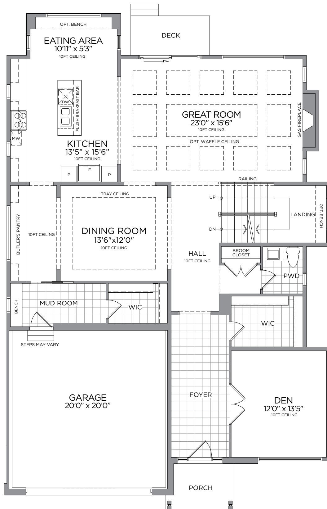
GROUND FLOOR ELEV. C
