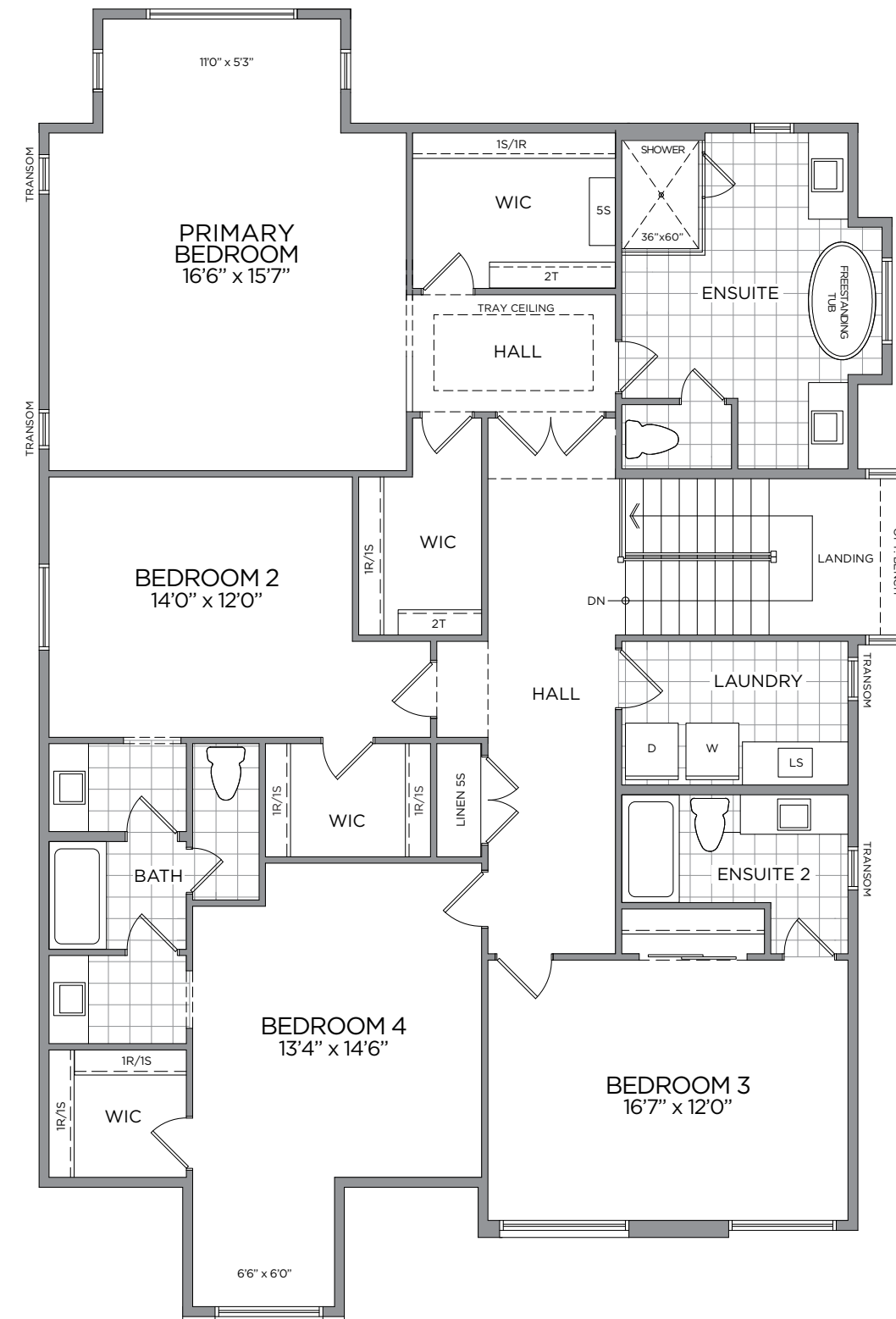
SECOND FLOOR ELEV. C
