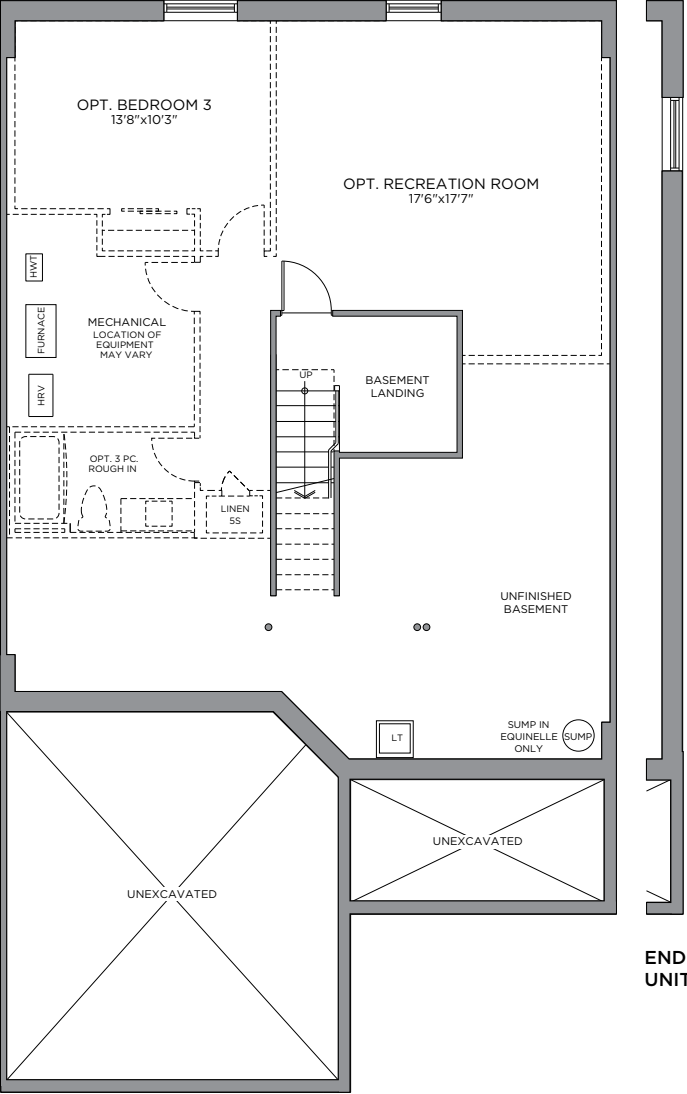
STANDARD BASEMENT PLAN OPTIONAL FINISHED BASEMENT PLAN 750 SQ. FT.
