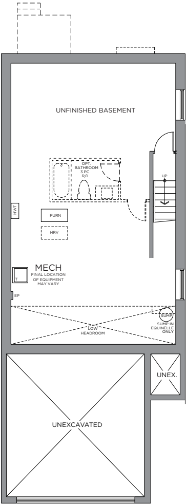
BASEMENT
