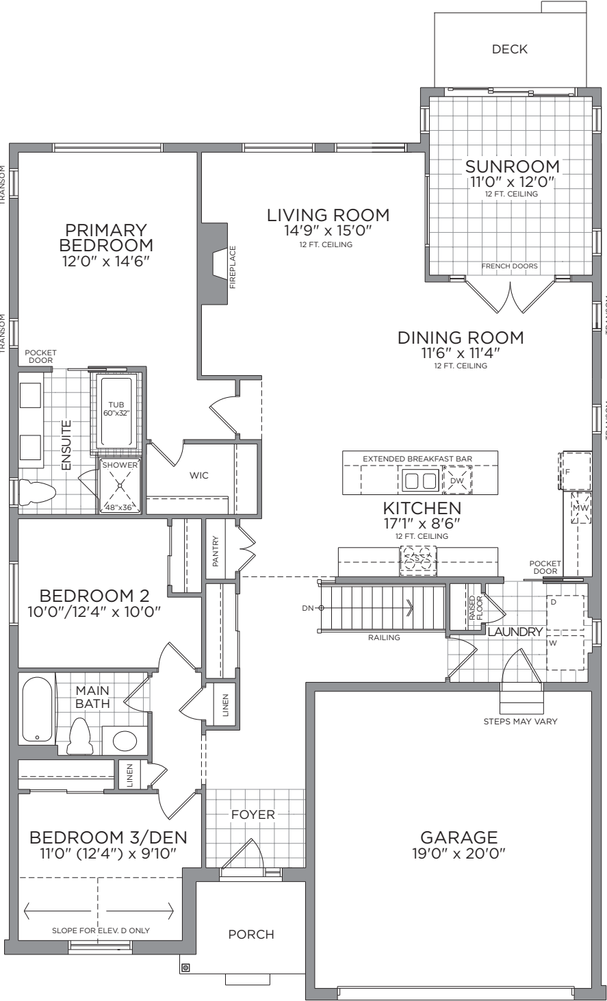
GROUND FLOOR
