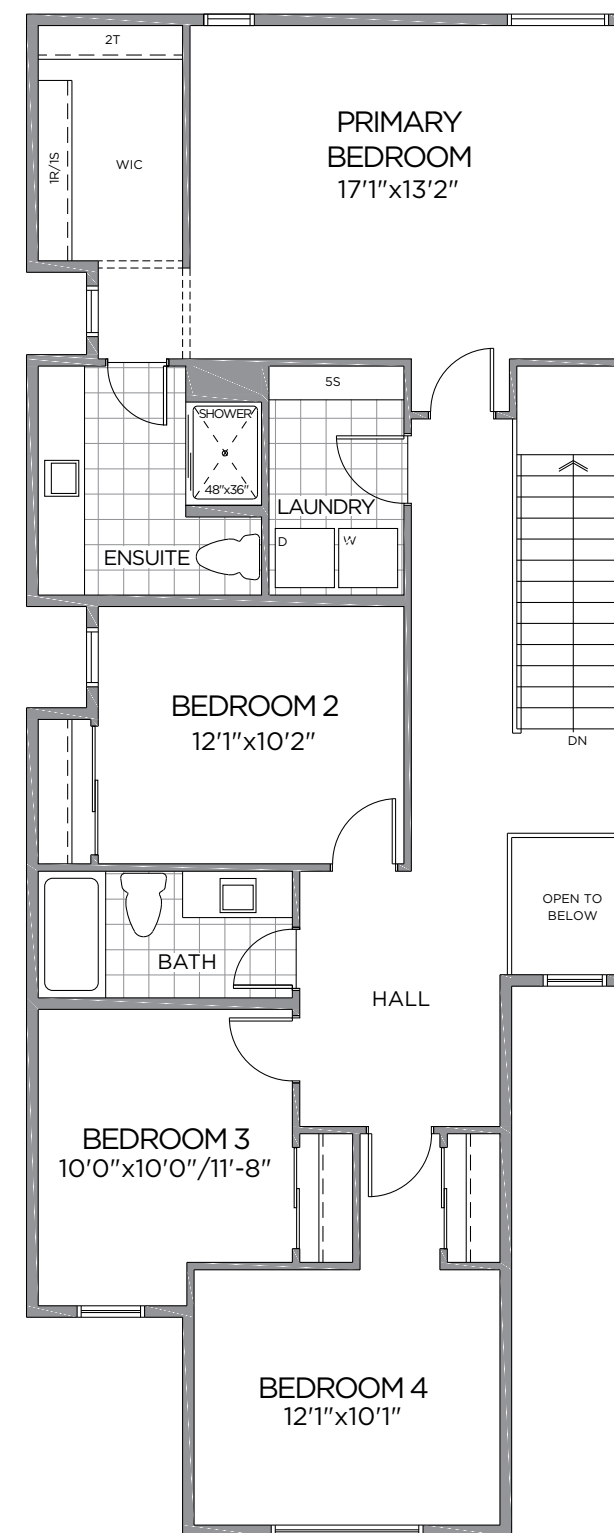
SECOND FLOOR ELEV. B/F
