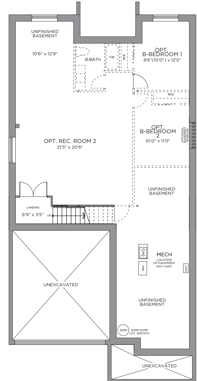
STANDARD BASEMENT PLAN OPT. FINISHED BASEMENT PLAN 1,104 SQ. FT.
