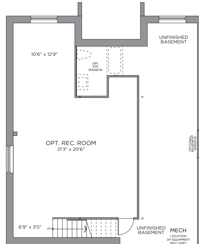
OPT. FINISHED BASEMENT REC. ROOM PLAN 707 SQ. FT.
