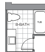
OPT. FINISHED BASEMENT BATHROOM 76 SQ. FT.
