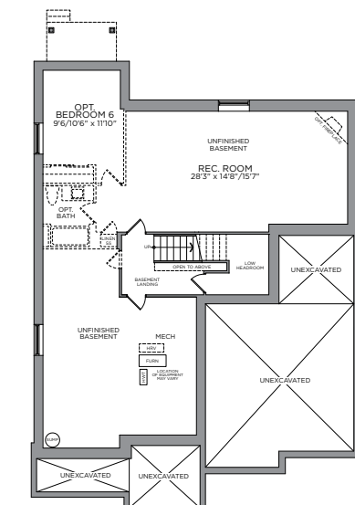
STANDARD BASEMENT OPT. FINISHED BASEMENT FINISHED AREA 852 SQ. FT.
