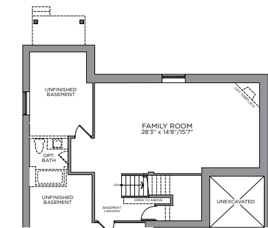
STANDARD BASEMENT OPT. FINISHED FAMILY ROOM FINISHED AREA 599 SQ. FT.
