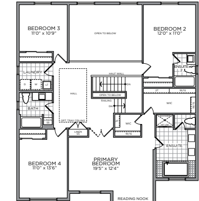
OPT. SECOND FLOOR ELEV. B -215 SQ. FT.
