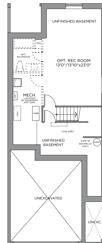
STANDARD BASEMENT ELEV. C OPT. FINISHED BASEMENT FINISHED AREA 468 SQ. FT.
