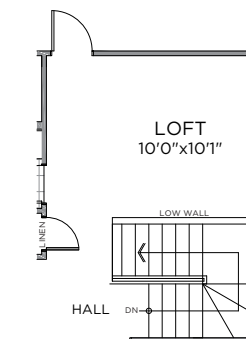
OPT. LOFT 98 SQ. FT.
