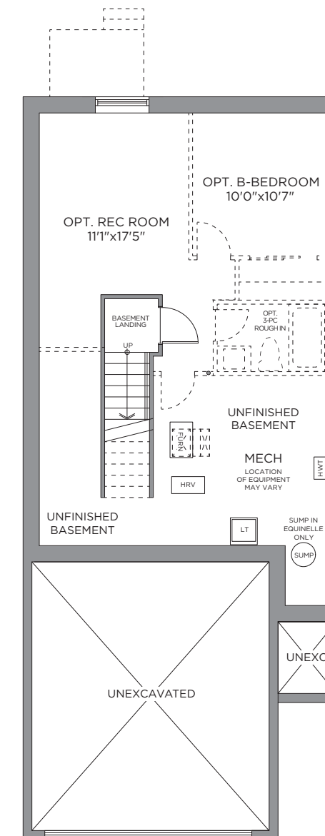
STANDARD BASEMENT PLAN OPT. FINISHED BASEMENT 480 SQ. FT.
