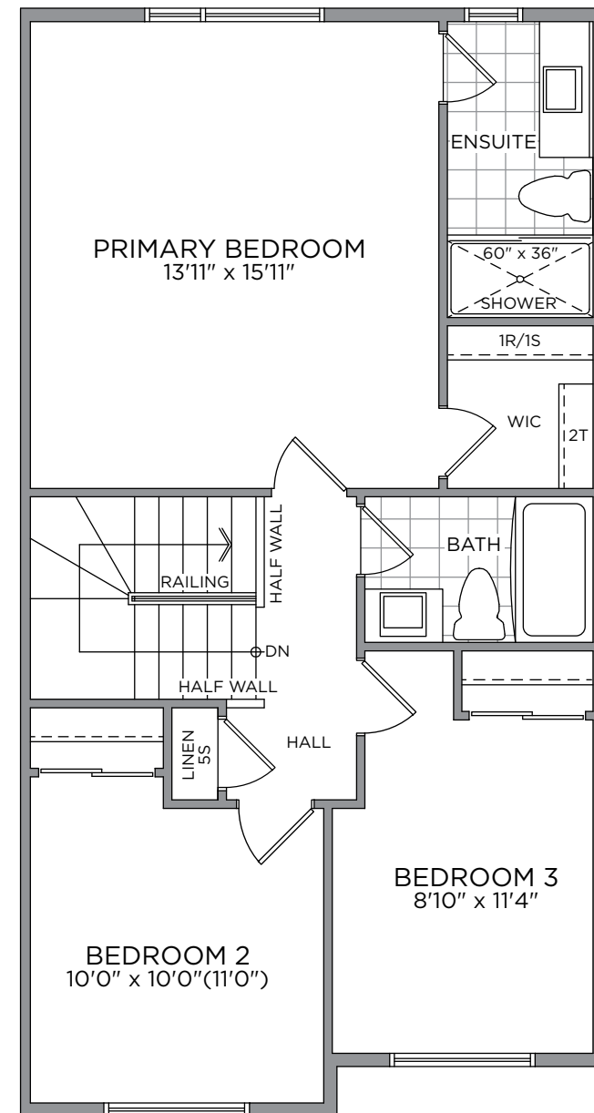
SECOND FLOOR
