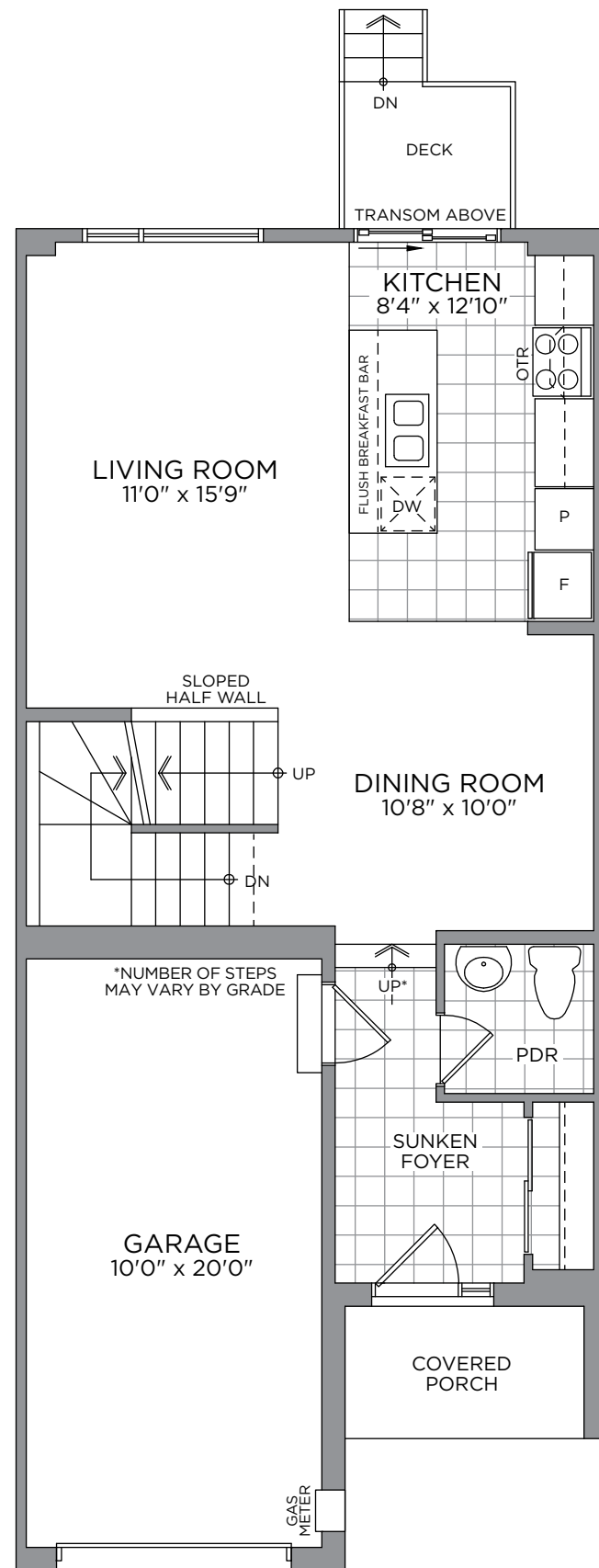
GROUND FLOOR
