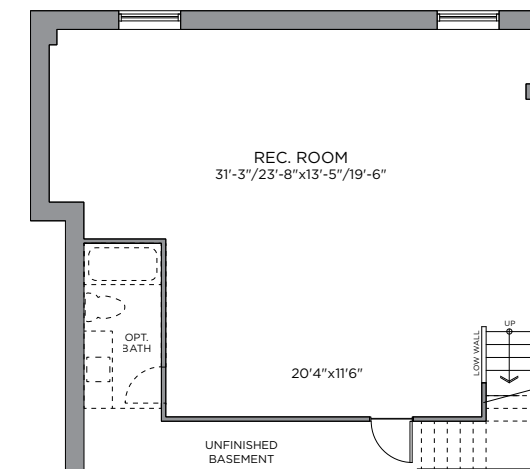
OPT. FINISHED BASEMENT REC. ROOM 769 SQ. FT.
