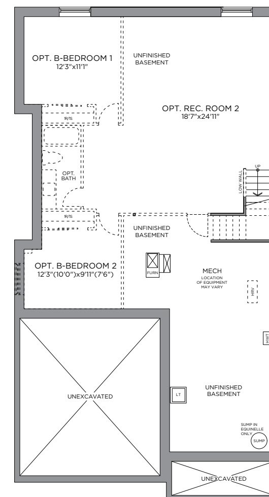
STANDARD BASEMENT PLAN OPT. FINISHED BASEMENT 1,015 SQ. FT.
