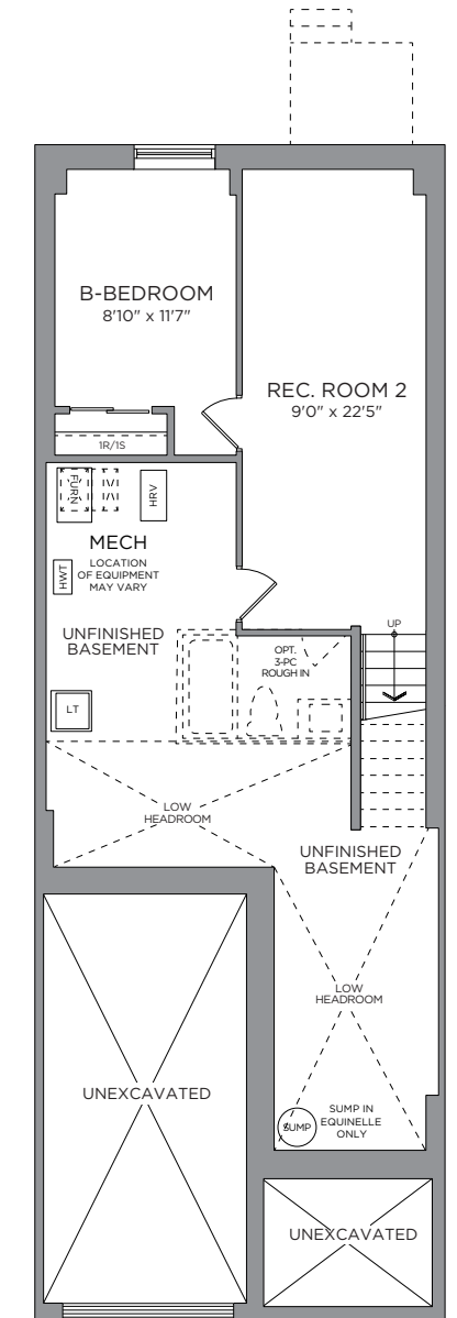
OPT. FINISHED BASEMENT REC. ROOM 2 & B-BEDROOM 397 SQ. FT.
