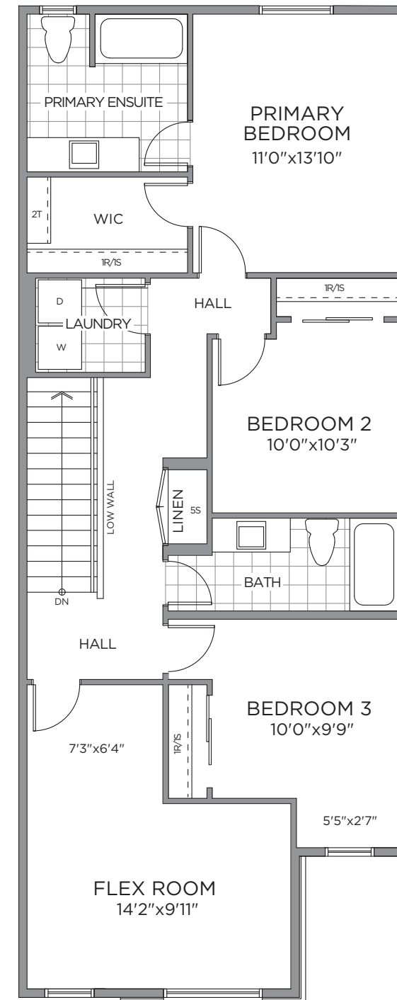
SECOND FLOOR
