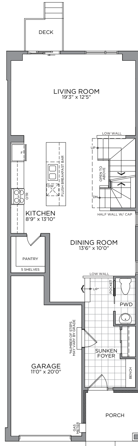
GROUND FLOOR
