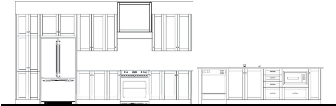
KITCHEN CABINET & ISLAND LAYOUT
