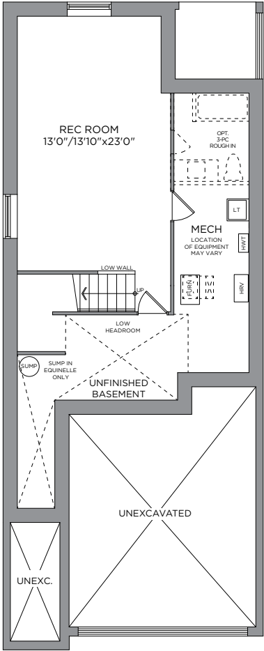
BASEMENT
