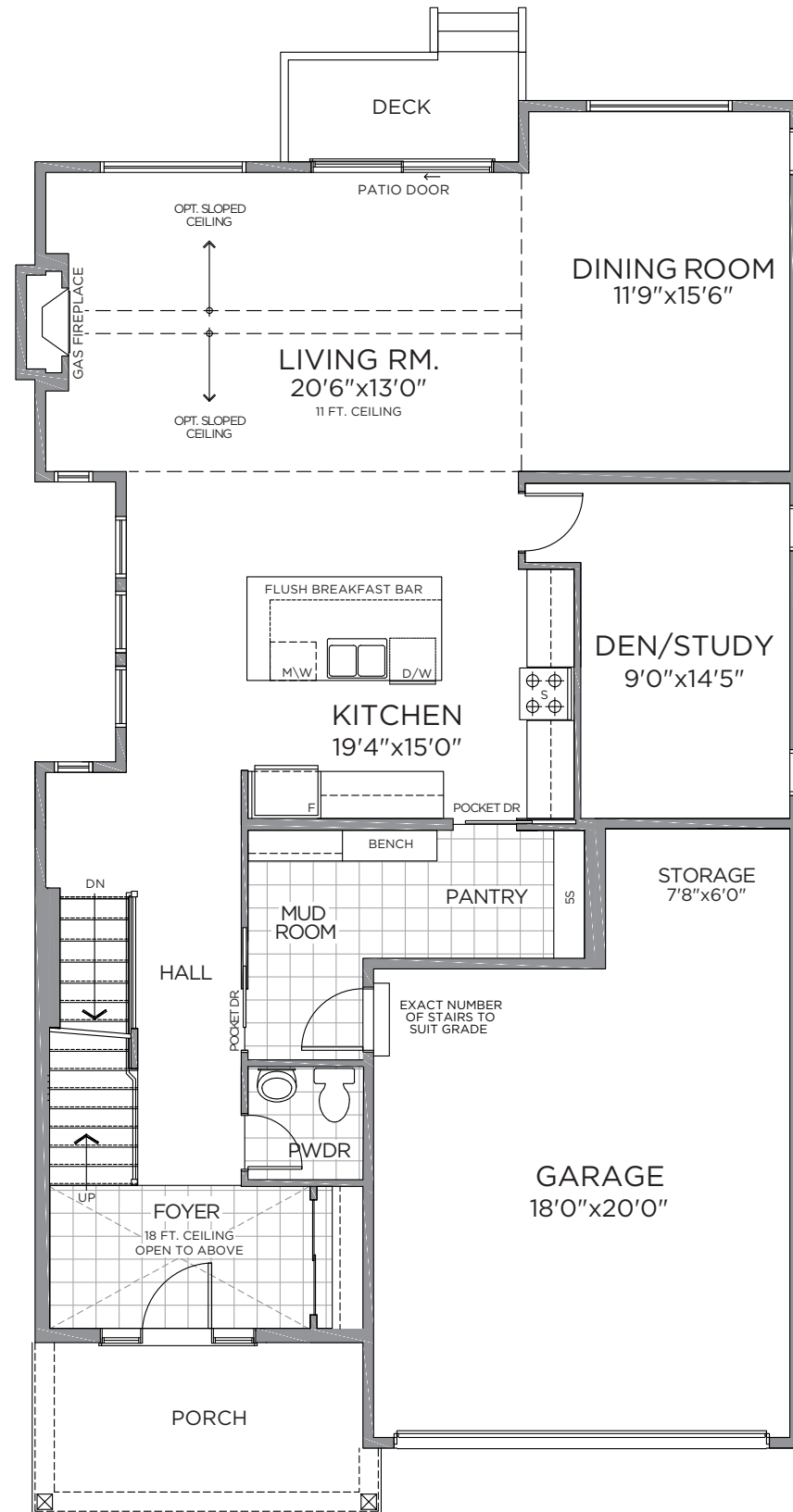
GROUND FLOOR
