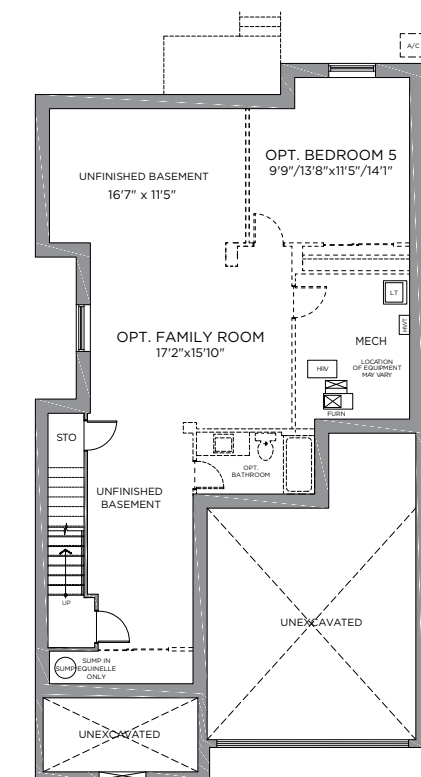
STANDARD BASEMENT OPT. FINISHED BASEMENT FINISHED AREA 1074 SQ. FT.
