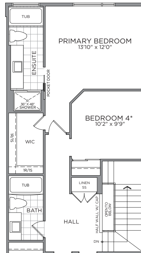
OPT. SECOND FLOOR
