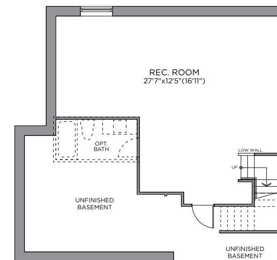
OPT. FINISHED BASEMENT REC. ROOM 582 SQ. FT.
