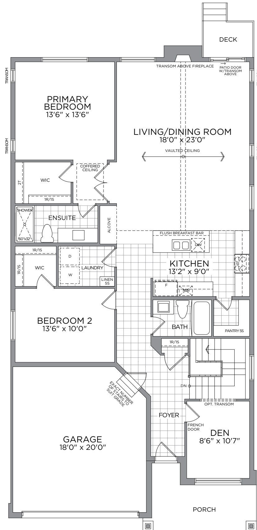
GROUND FLOOR
