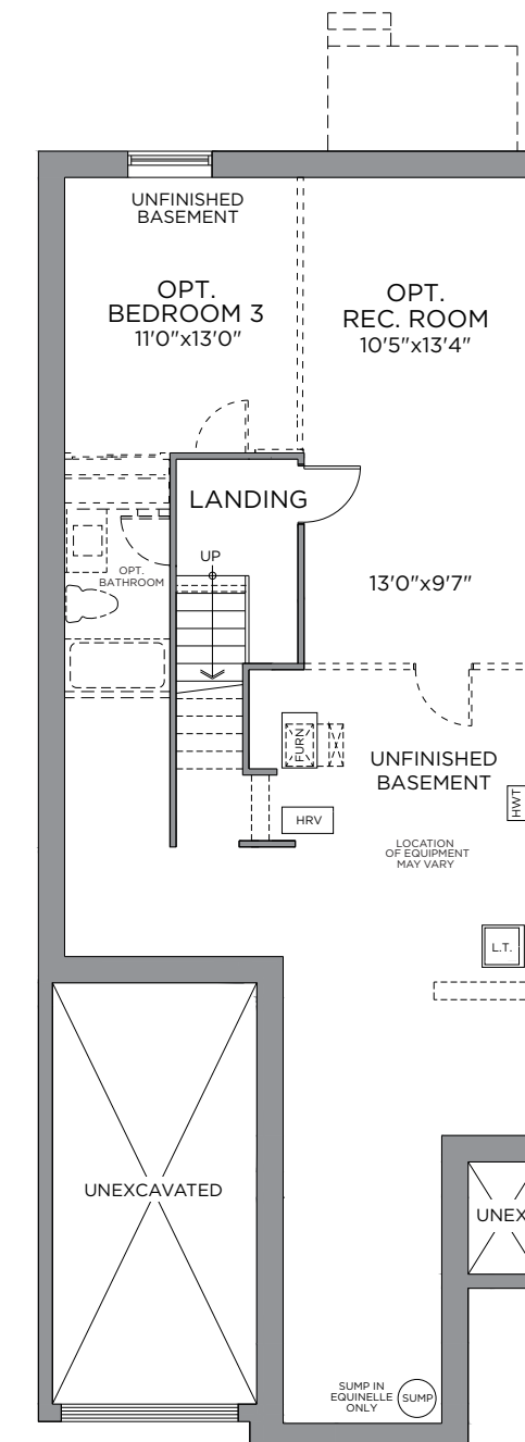
BASEMENT PLAN ELEV. 'B' OPTIONAL FINISHED BASEMENT PLAN 594 SQ. FT.
