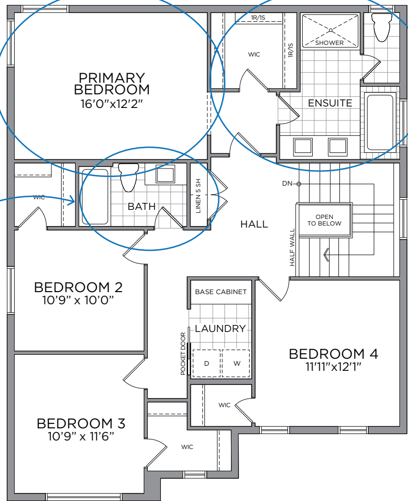
SECOND FLOOR
