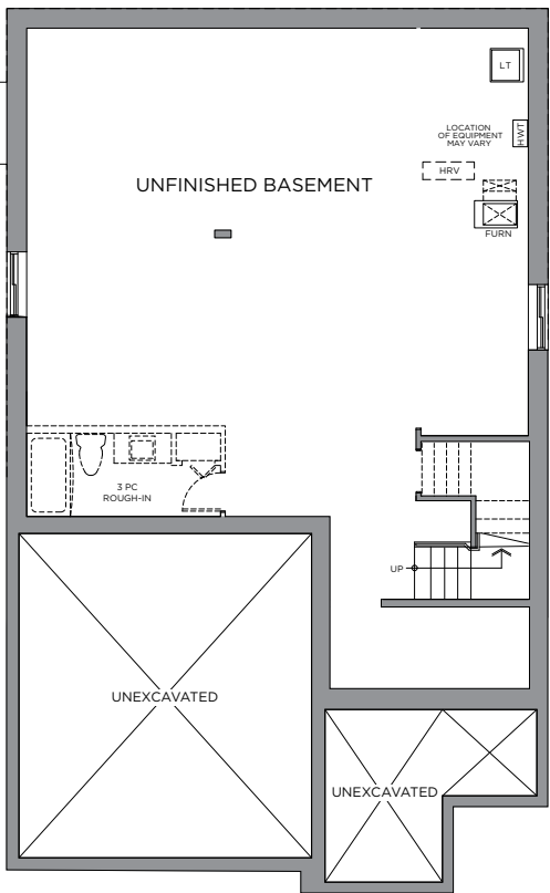
STANDARD BASEMENT
