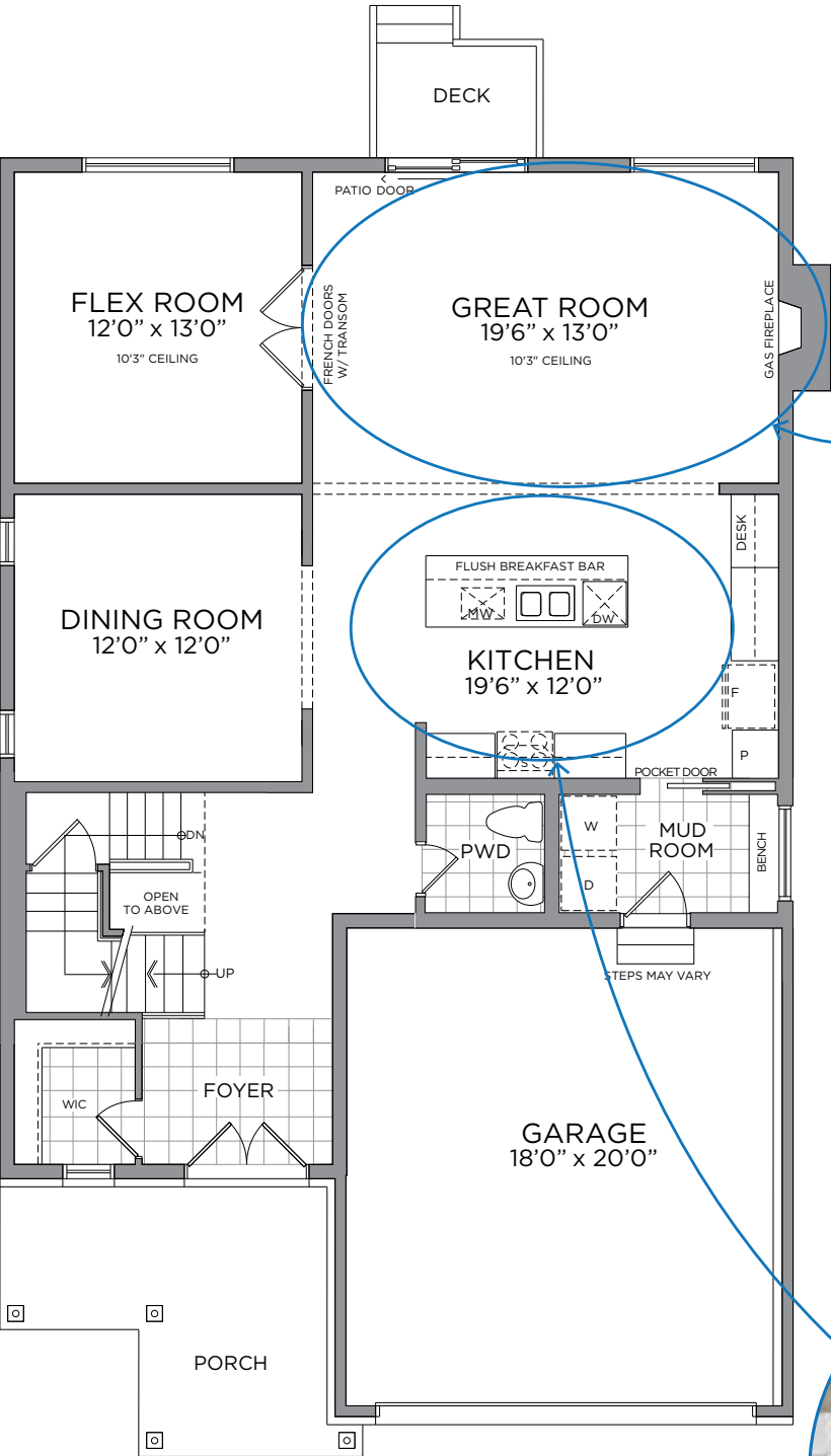
GROUND FLOOR
