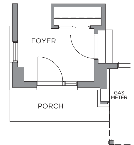
GROUND FLOOR PLAN END UNIT
