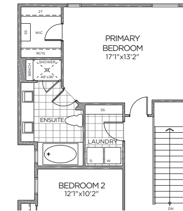
OPT. PRIMARY ENSUITE ELEV. B
