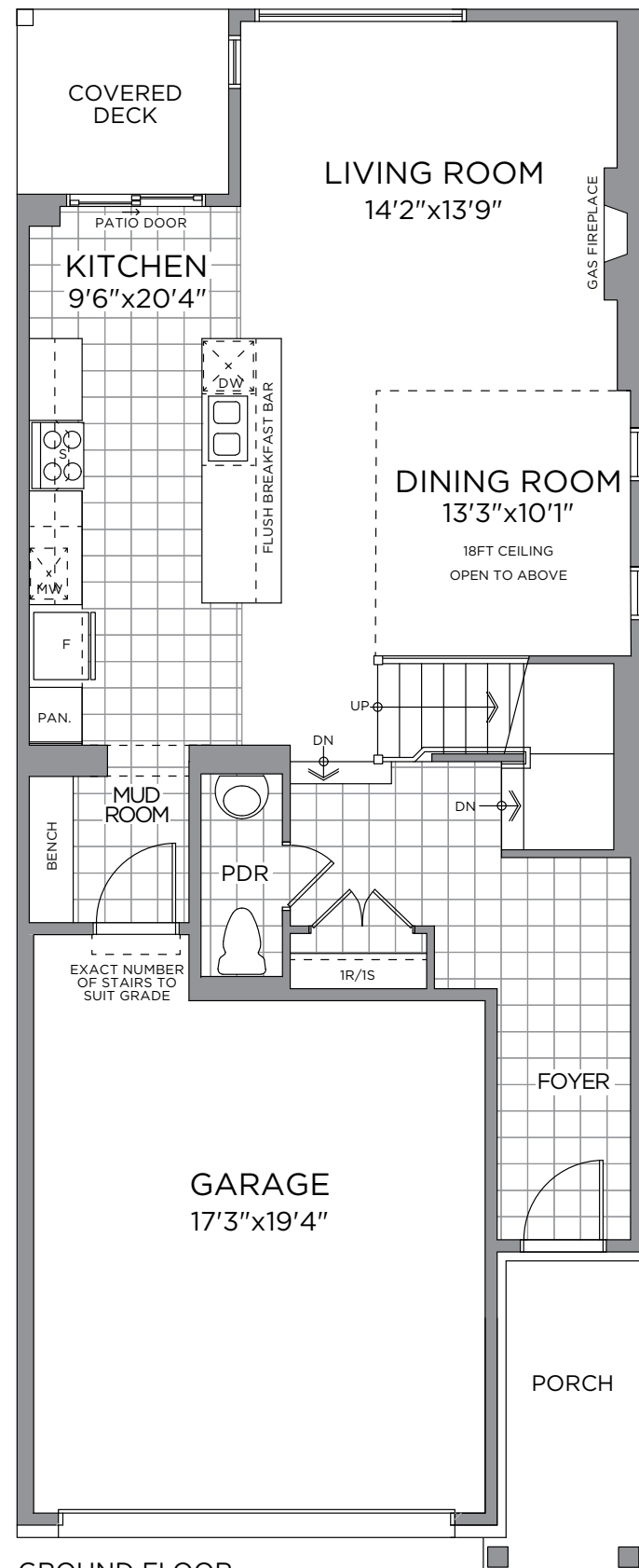
GROUND FLOOR
