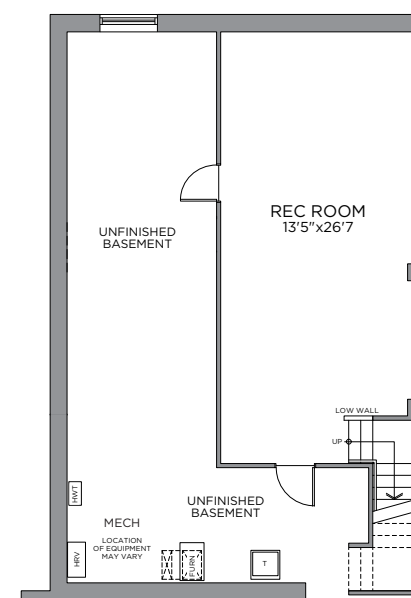
OPT. FINISHED BASEMENT REC. ROOM PLAN 455 SQ. FT.
