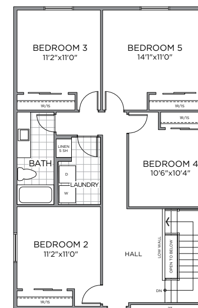
OPT. SECOND FLOOR 5 BEDROOM PLAN + 191 SQ. FT. ELEV. B (CLOSES OFF THE 2-STOREY CEILING IN THE LIVING ROOM)
