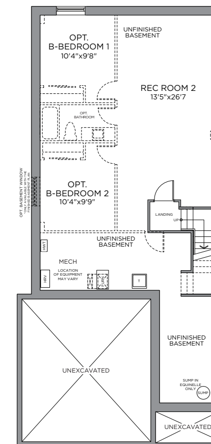
STANDARD BASEMENT OPT. FINISHED BASEMENT PLAN 818 SQ. FT.
