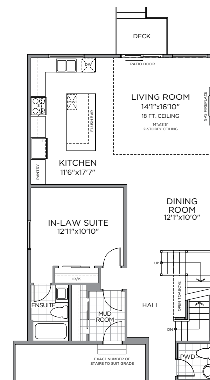
OPT. GROUND FLOOR W/ IN-LAW SUITE ELEV. B
