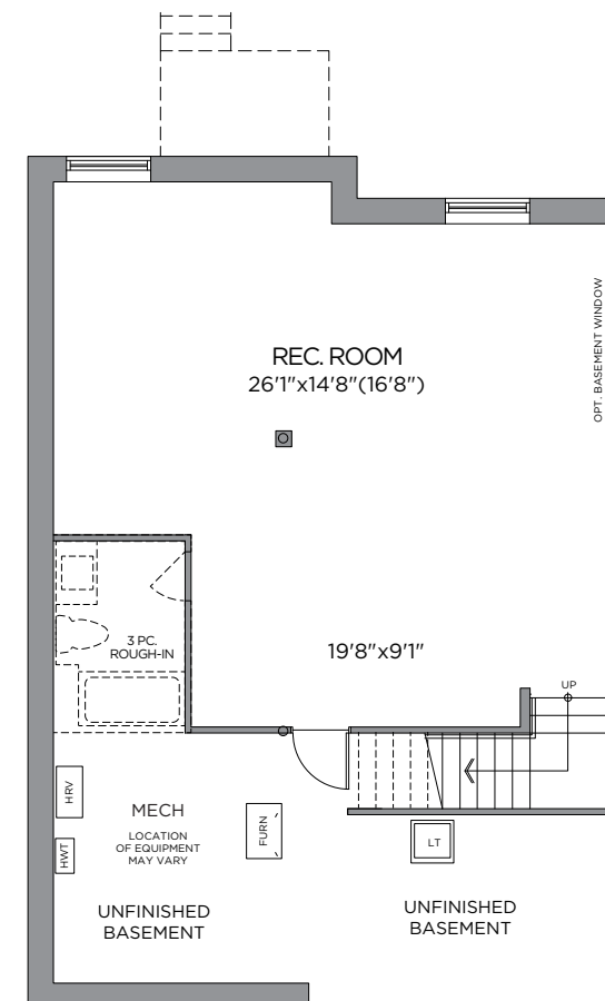
OPT. FINISHED BASEMENT REC. ROOM 683 SQ. FT.
