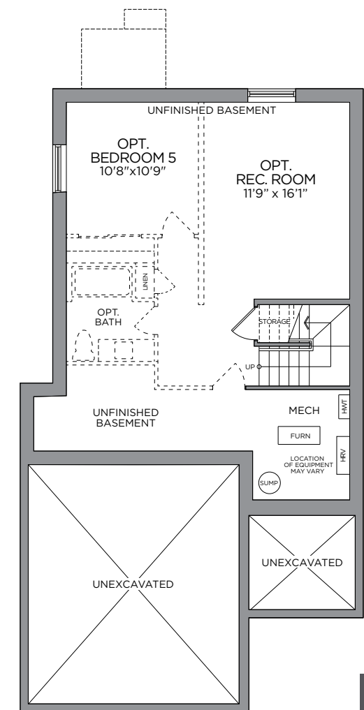
STANDARD BASEMENT PLAN OPT. FINISHED BASEMENT PLAN 559 SQ. FT.
