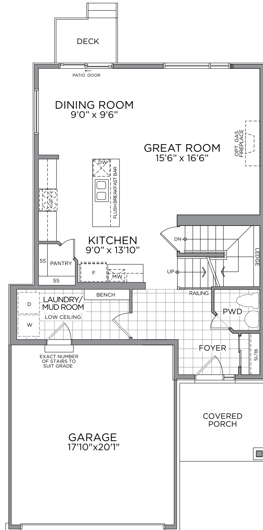
GROUND FLOOR
